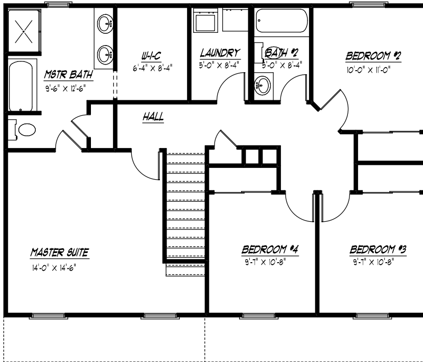
SECOND FLOOR FRAMING PLAN
