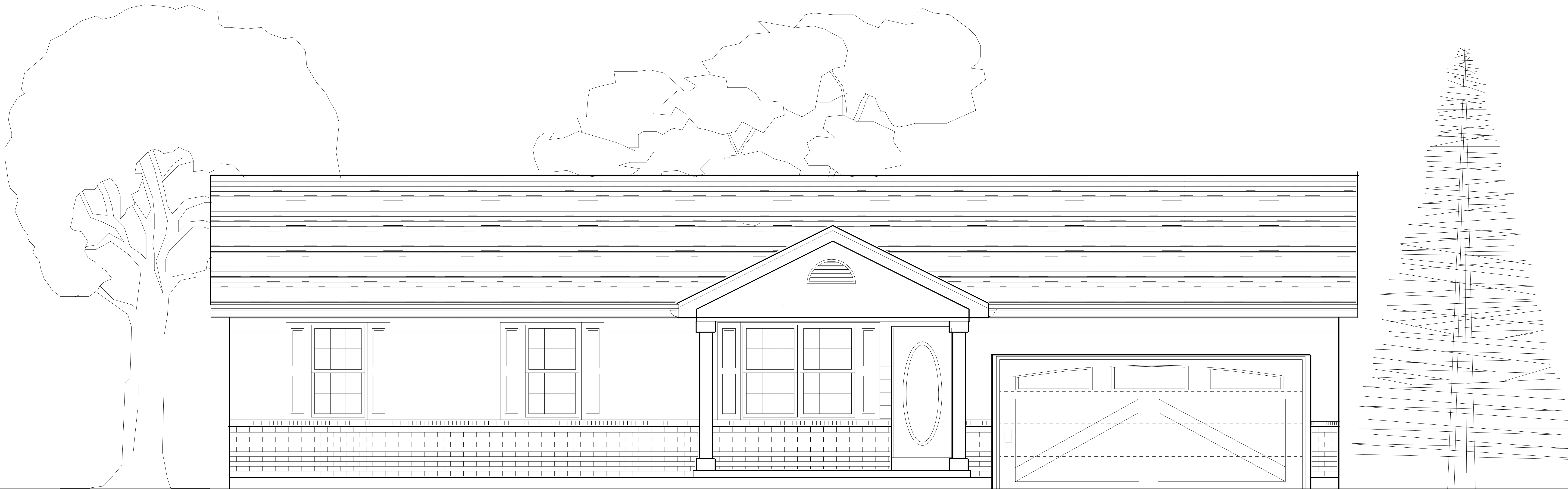
FRONT ELEVATION 'B'
